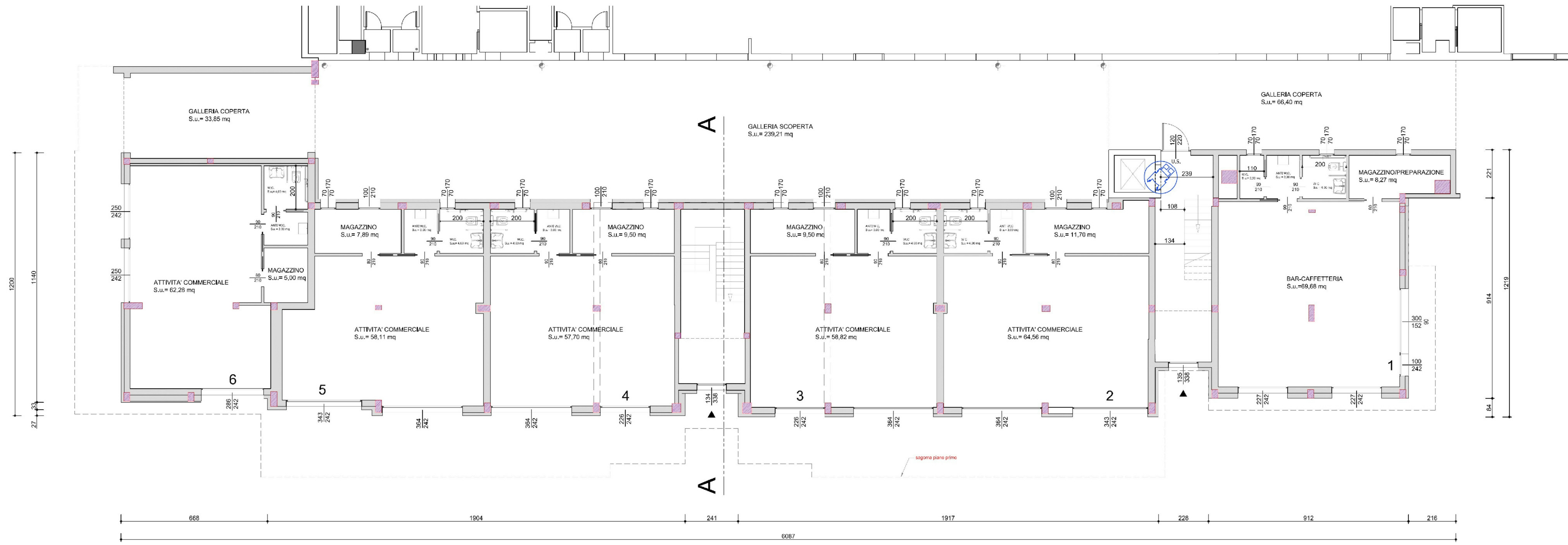
PIANO TERRA
