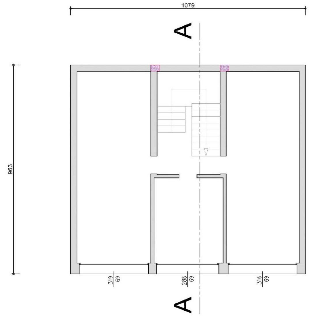
PIANO INTERRATO
